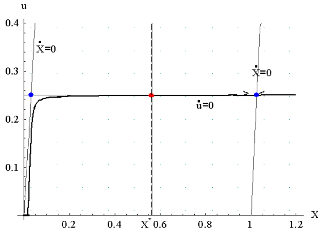
Figure 3: Isoclines and saddle paths for the case a = 2, \beta = 0.25, c = 2, \gamma = 0.45, r = 0.05, \rho = 0.02
